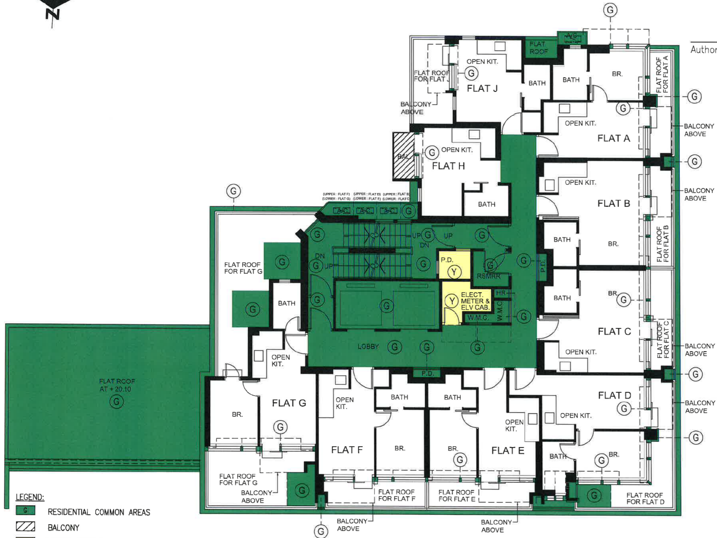
3RD FLOOR PLAN (FOR IDENTIFICATION PURPOSE ONLY) (NOT TO SCALE)
